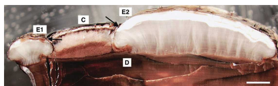
Fig. 4. Transverse section of the enamel bands. C: cementum, D: dentin, E1: enamel (narrow), E2: enamel (wide). Arrows: CEJ. Scale bar: 1 mm
