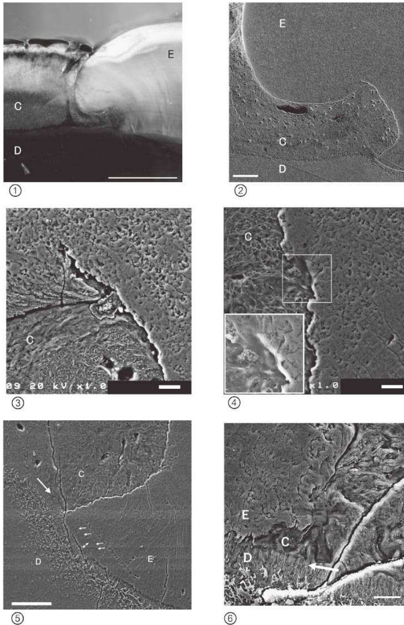
Fig. 8. (①: Reflected light microscopy, ②-⑥: SEM image)
