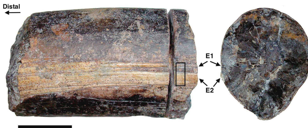
Fig. 2. Kitashiogo C specimen: (Ibaraki Nature Museum: INM-4-013796). Lateral (left) and mesial (right) view. E1: enamel band (narrow), E2: enamel band (wide). Box: area of Fig.3 (cementum sandwiched between two bands of the enamel). Scale bar: 30 mm
