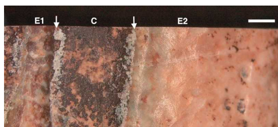
Fig. 3. Surface of the enamel band. C: cementum, E1: enamel (narrow), E2: enamel (wide). Arrows: CEJ. Scale bar: 1 mm
