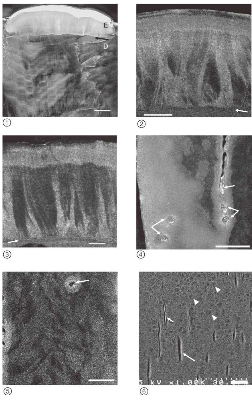
Fig. 5. (①-⑤: Reflected light microscopy, ⑥: SEM image)
