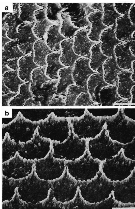
Fig. 9. SEM images of enamel prisms of molar of Stegolophodon pseudolatidens (Miocene, Kitashiogo, Ibaraki Prefecture, Japan).
