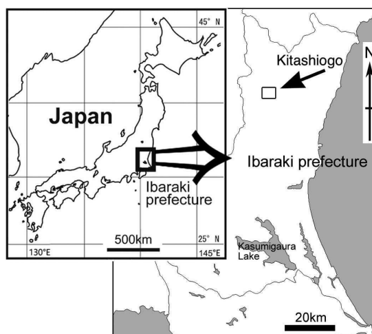
Fig. 1. Map showing the locality of the specimen (Kitashiogo C specimen). Topographical map “Hitachiomiya”, 1:50,000 in scale by the Geographical Survey Institute of Japan.
